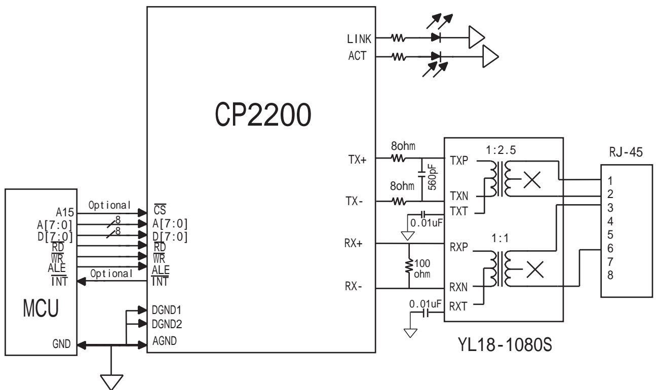
Typical Connection Diagram
