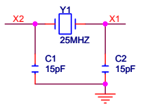
CLOCK
